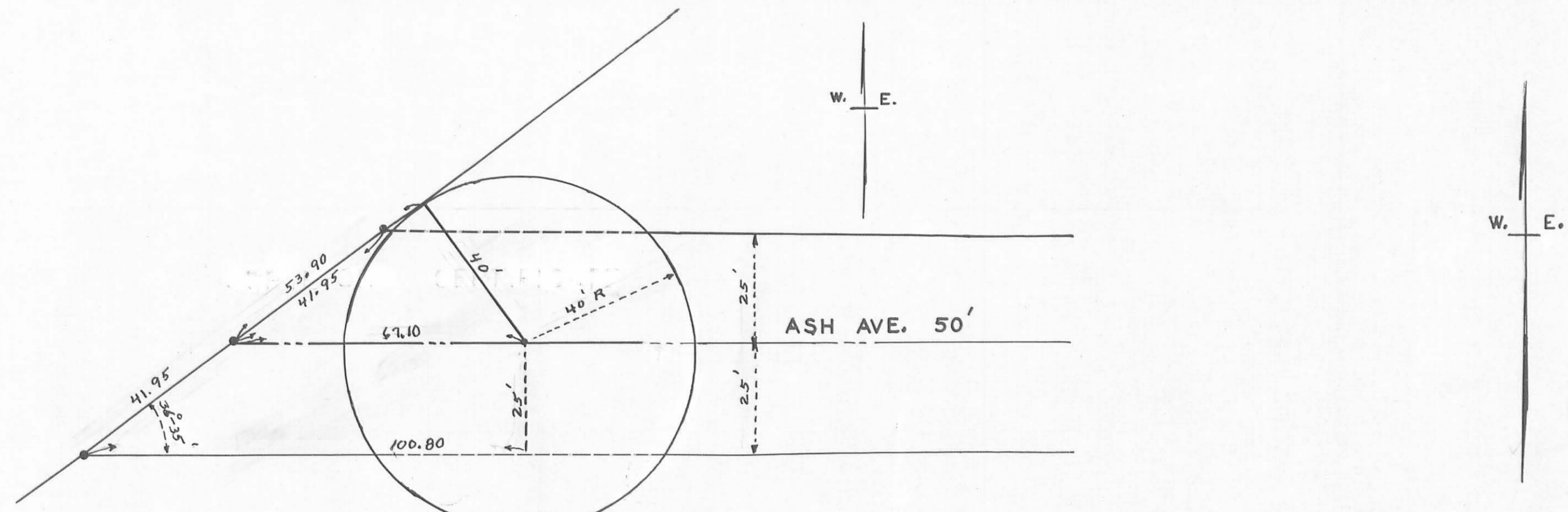
CUL-DE-SAC DETAIL 1" = 25'
